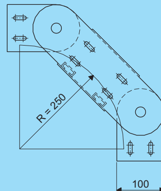
vertical bend piece as vertical outer bend
