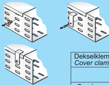
montage-toepassing mounting application
