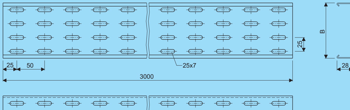
Kabelkanaal - H28R Cable duct - H28R
