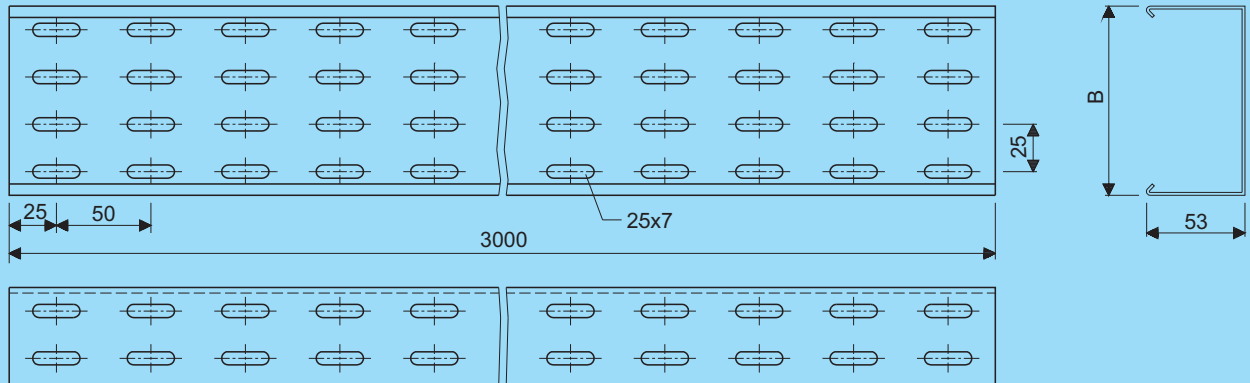
Kabelkanaal - H53R Cable duct - H53R
